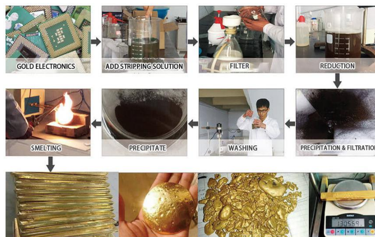
3-18. Figure_ Flow chart precious metal recovery [ https://www.alibaba.com/ ]
