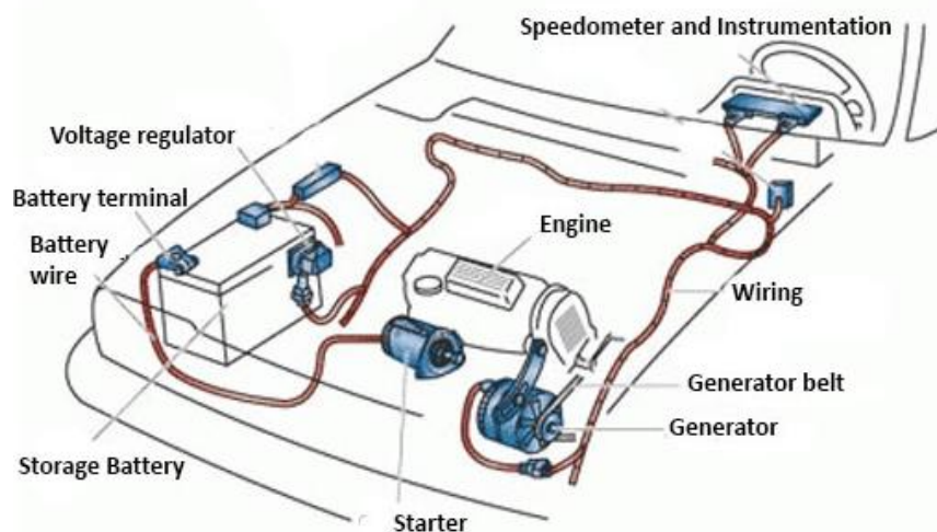
3-13. Figure_ Vehicle electrical system construction
