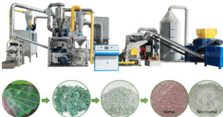
6-8. Figure_ Technology for obtaining powders from metals and non-metals
